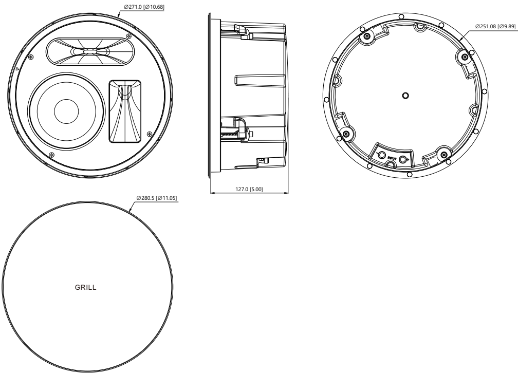
X6 Finished product dimensions
